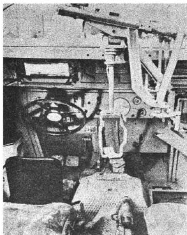
Interior of the half-track at left shows its unique inverted steering wheel. Included among instruments on the dashboard is a tachometer, indicating engine revolutions.
