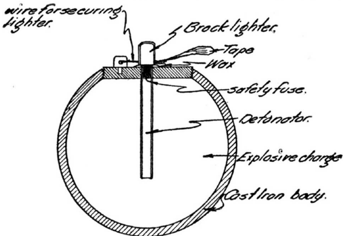
SECTION. Diameter of Grenade 3"
